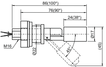
IL-BA-H-P16-P(IL-BA-H-F16-F)
